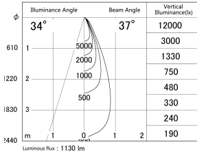
■ Direct Horizontal Illuminance DD155-1035MW9027-FX
