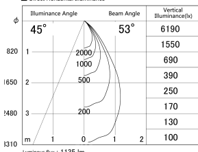
■ Direct Horizontal Illuminance DD155-1055MW9027-FX
