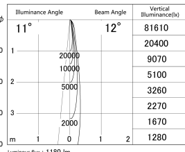
■ Direct Horizontal Illuminance DD155-1510MW9027-FX
