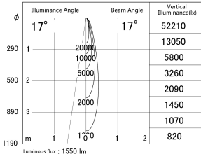
■ Direct Horizontal Illuminance DD155-1515MW9027-FX
