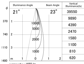
■ Direct Horizontal Illuminance DD155-1525MW9027-FX
