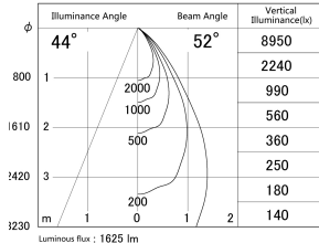
■ Direct Horizontal Illuminance DD155-1555MW9027-FX
