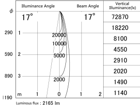
■ Direct Horizontal Illuminance DD155-2015MW9027-FX
