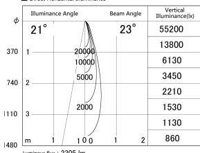
■ Direct Horizontal Illuminance DD155-2025MW9027-FX
