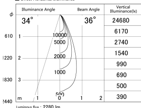
■ Direct Horizontal Illuminance DD155-2035MW9027-FX
