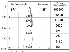
■ Direct Horizontal Illuminance DD155-2525MW9027-FX
