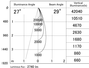
■ Direct Horizontal Illuminance DD155-2530MW9027-FX
