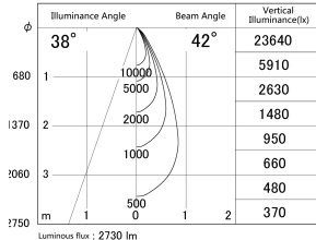
■ Direct Horizontal Illuminance DD155-2540MW9027-FX
