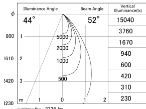
■ Direct Horizontal Illuminance DD155-2555MW9027-FX
