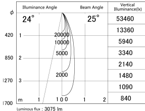
■ Direct Horizontal Illuminance DD155-3025MW9027-FX
