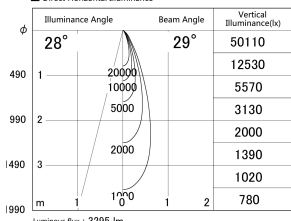
■ Direct Horizontal Illuminance DD155-3030MW9027-FX
