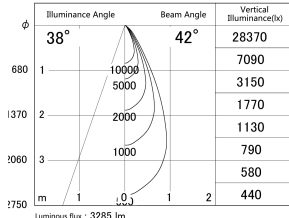
■ Direct Horizontal Illuminance DD155-3040MW9027-FX
