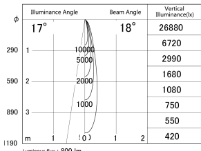
■ Direct Horizontal Illuminance DD155-0815MW9030-FX
