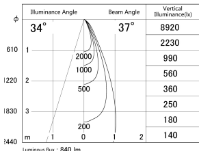
■ Direct Horizontal Illuminance DD155-0835MW9030-FX
