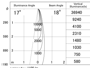
■ Direct Horizontal Illuminance DD155-1015MW9030-FX
