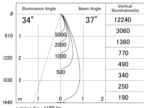
■ Direct Horizontal Illuminance DD155-1035MW9030-FX
