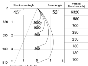
■ Direct Horizontal Illuminance DD155-1055MW9030-FX
