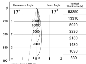
■ Direct Horizontal Illuminance DD155-1515MW9030-FX
