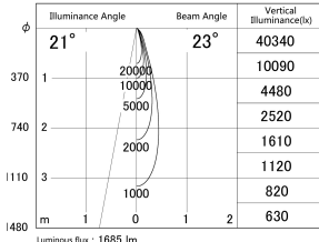
■ Direct Horizontal Illuminance DD155-1525MW9030-FX
