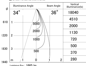
■ Direct Horizontal Illuminance DD155-1535MW9030-FX
