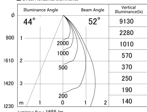
■ Direct Horizontal Illuminance DD155-1555MW9030-FX
