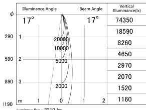
■ Direct Horizontal Illuminance DD155-2015MW9030-FX
