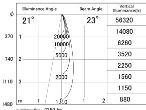
■ Direct Horizontal Illuminance DD155-2025MW9030-FX
