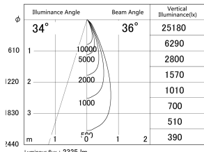
■ Direct Horizontal Illuminance DD155-2035MW9030-FX
