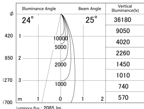
■ Direct Horizontal Illuminance DD155-2515MW9030-FX
