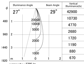
■ Direct Horizontal Illuminance DD155-2530MW9030-FX
