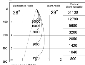
■ Direct Horizontal Illuminance DD155-3030MW9030-FX
