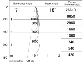
■ Direct Horizontal Illuminance DD155-0815MW9035-FX
