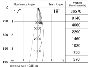
■ Direct Horizontal Illuminance DD155-1015MW9035-FX
