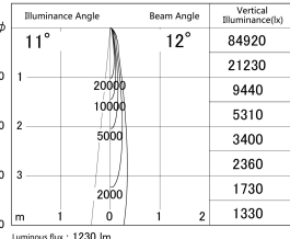
■ Direct Horizontal Illuminance DD155-1510MW9035-FX
