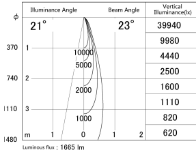
■ Direct Horizontal Illuminance DD155-1525MW9035-FX
