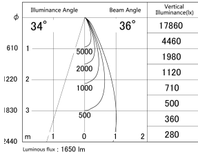
■ Direct Horizontal Illuminance DD155-1535MW9035-FX
