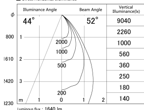
■ Direct Horizontal Illuminance DD155-1555MW9035-FX
