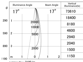
■ Direct Horizontal Illuminance DD155-2015MW9035-FX
