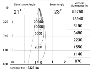
■ Direct Horizontal Illuminance DD155-2025MW9035-FX
