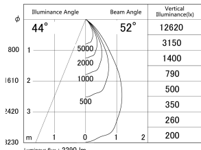
■ Direct Horizontal Illuminance DD155-2055MW9035-FX
