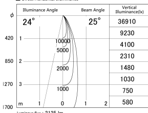
■ Direct Horizontal Illuminance DD155-2515MW9035-FX
