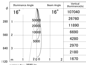
■ Direct Horizontal Illuminance DD155-2525MW9035-FX
