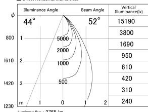
■ Direct Horizontal Illuminance DD155-2555MW9035-FX
