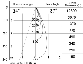
■ Direct Horizontal Illuminance DD155-1035MW9040-FX
