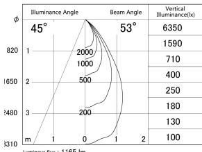
■ Direct Horizontal Illuminance DD155-1055MW9040-FX
