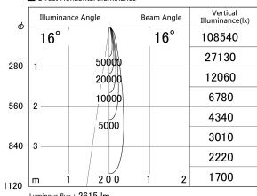
■ Direct Horizontal Illuminance DD155-2525MW9040-FX
