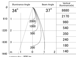
■ Direct Horizontal Illuminance DD155-0835DW9027-FX
