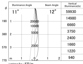
■ Direct Horizontal Illuminance DD155-1010DW9027-FX
