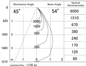
■ Direct Horizontal Illuminance DD155-1055DW9027-FX
