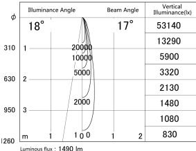
■ Direct Horizontal Illuminance DD155-1515DW9027-FX
